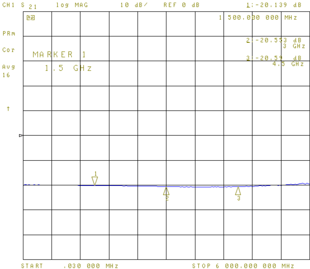
20dB Attenuator, S21
