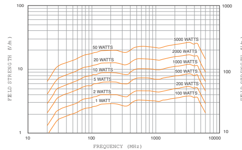
ATR26M 6G FIELD STRENGTH MEASURED AT THREE METERS
