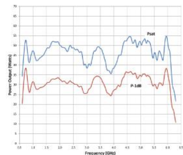
30/2051G188 TYPICAL POWER OUTPUT WITH 0.7-6.0GHz BAND SELECTED
