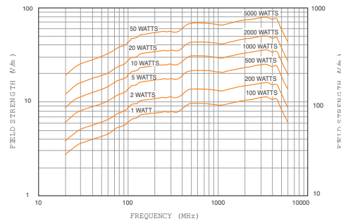
ATR26M 6G FIELD STRENGTH MEASURED AT ONE METER
