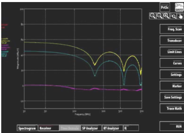
Fig. 1 – Measurement of an impulse with excellent dynamic range (Peak, Quasi-Peak, Average).
