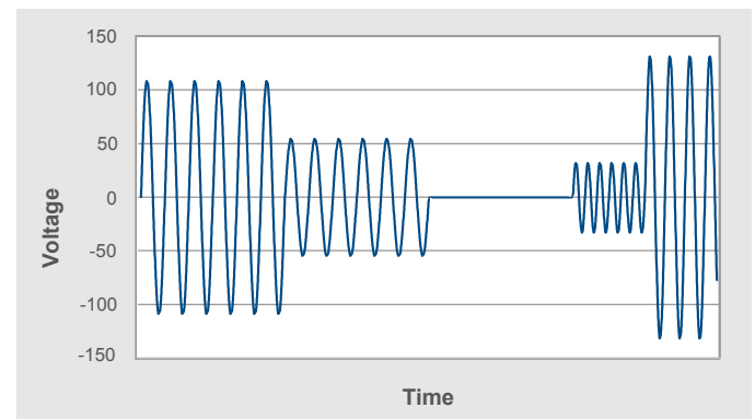
Figure 6 - Voltage/Frequency Variation
