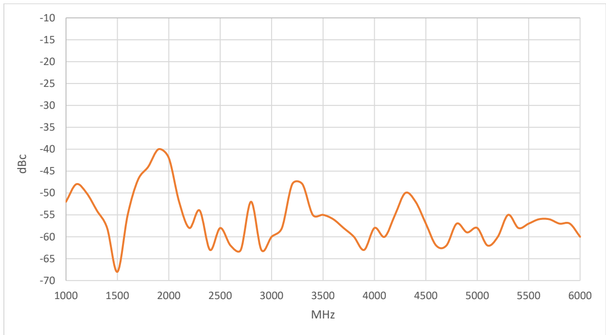
TYPICAL 3 RD HARMONIC @ 400 W
