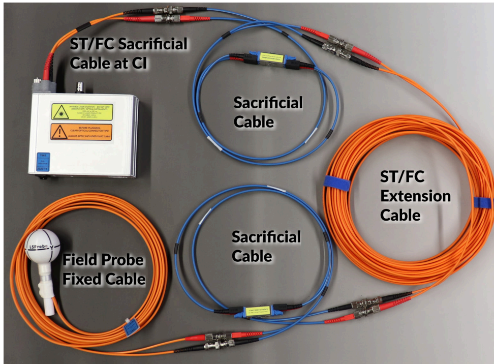
Figure 5: Typical LSProbe 1.2 Field Probe System with sacrificial cable kits
