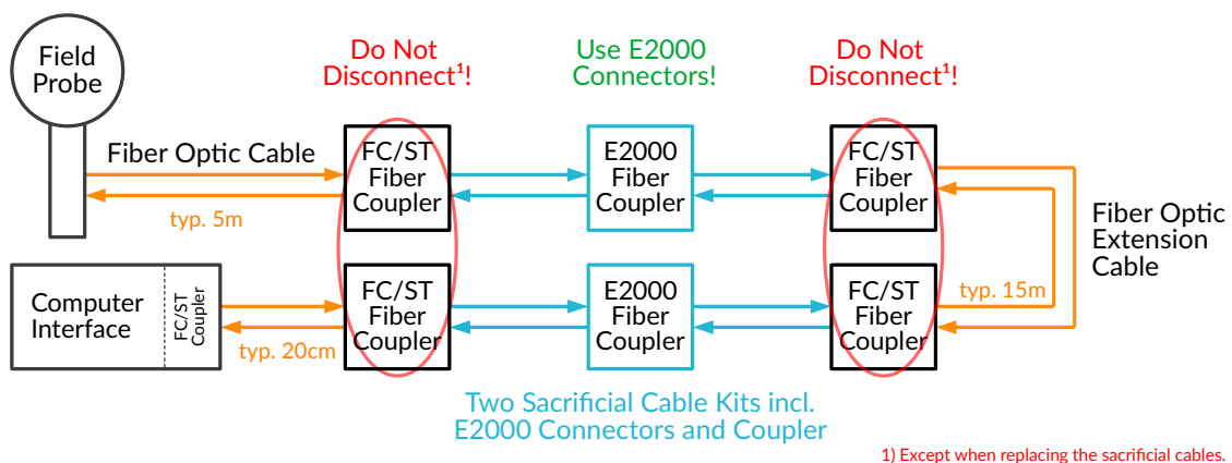
Figure 6: Fiber connections of a typical LSProbe 1.2 Field Probe System
