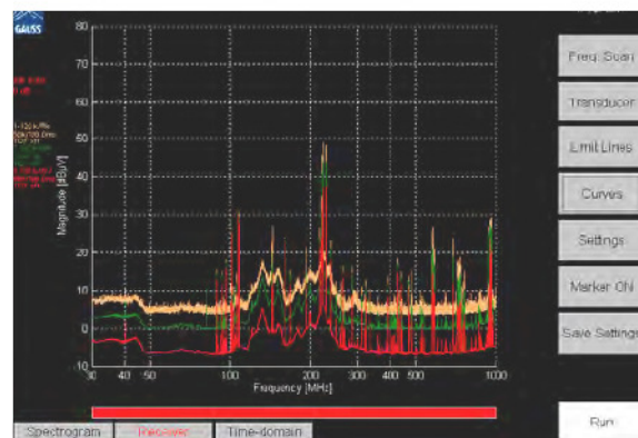
Fig. 23 – Measurement of ambient noise in the frequency range from 30 MHz to 1 GHz.
