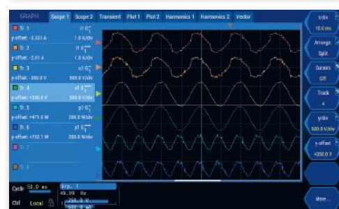
Display of sampling values in two scopes
