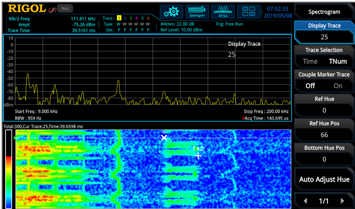
Figure 9: Interference measurement of power supply with acq. time of 143 μsec and Z marker evaluation
