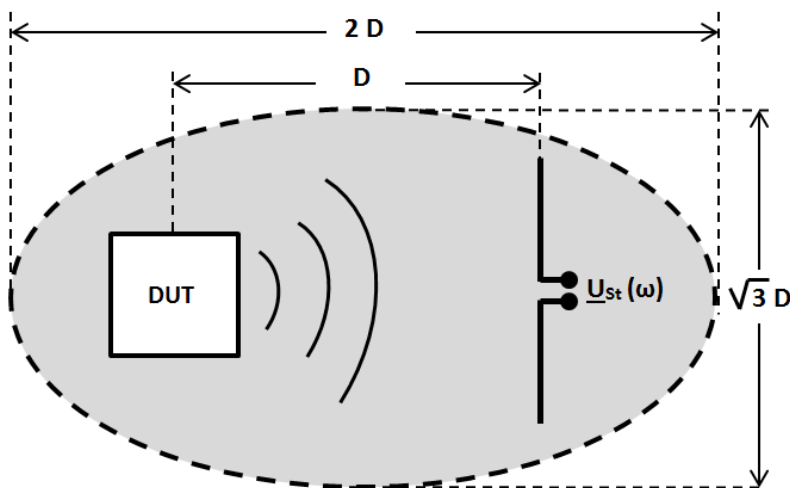
Figure 12: free field measurement for radiated emission
