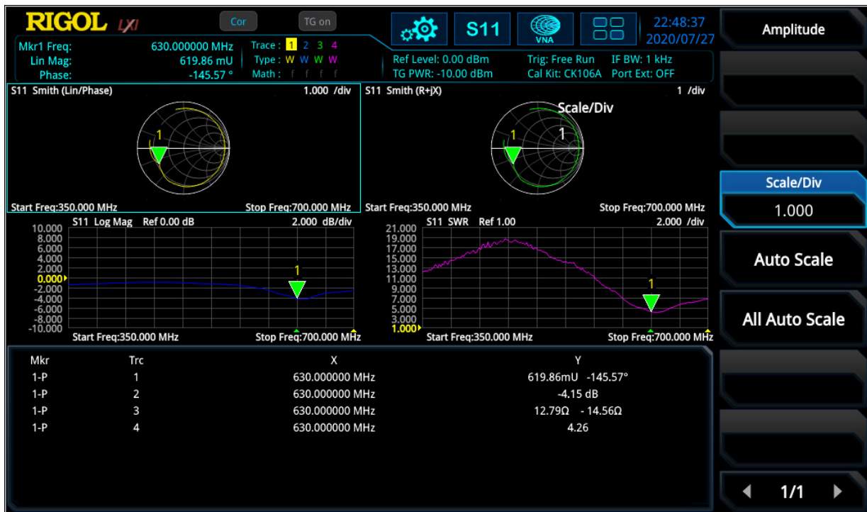
Figure 17: VNA Mode with different window of S 11 parameter like smith- and Polar Plane, logarithm. Magnitude and SWR
