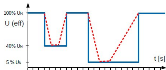
Fig.2: Voltage fluctuation
