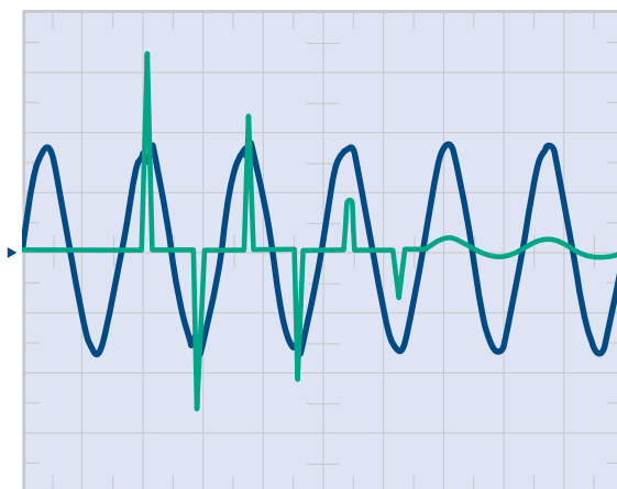
10.000 mS/div Wf1, Chn 001, 100 V/div. Wf2, Chn 002, 20 A/div. Fig. 6 - Start-Up Inrush Current Macro
