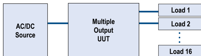
Figure 1(b) - Distributed Measurements: showing how a multi-output UUT & AC/DC source would be connected with one 4300 chassis. If UUT outputs are 8 or less, additional UUTs could be tested in parallel with addition of Power Analyzers.
