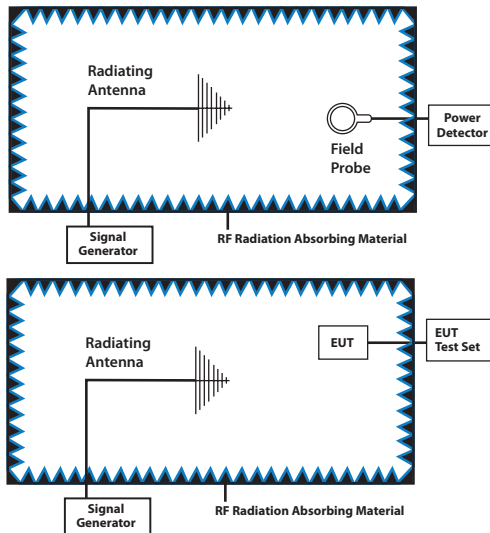
Figure 7.3.3. The Substitution Method Diagram
