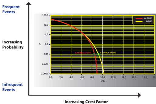
Figure 6.3.2. Dual CCDF: amplifier input (yellow), and amplifier output (red)
