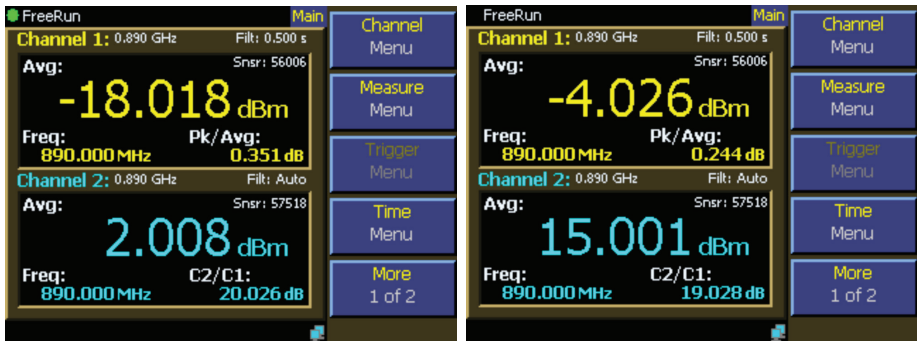
Figure 8.3.4. Two-Channel measurements showing amplifier gain (Channel 2 to Channel 1 ratio) dropping by 1dB
