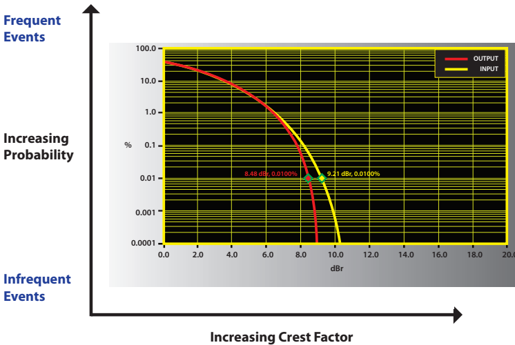
Figure 6.3.6 Normalized CCDF plot showing probability on the Y axis versus normalized power on the X axis (dual channel overlay)
