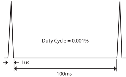
Figure 7.1.4. Narrow Duty Cycle pulse envelope
