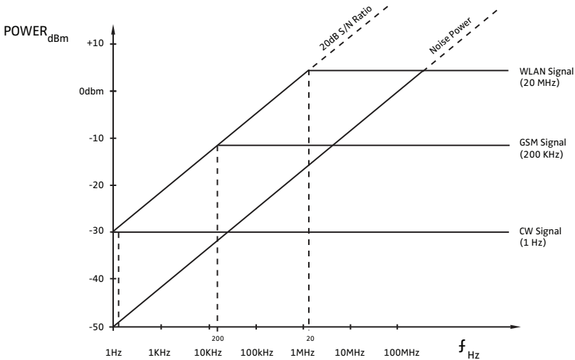
8.1.1 Graph of average noise power versus noise bandwidth, showing how BW may be reduced to improve S/N
