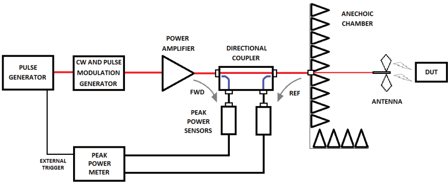
Figure 7.3.4. Accurate Monitoring of delivered power
