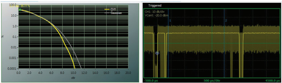
Figure 6.2.6. Screen shots showing cursor measurements and statistical distributions
