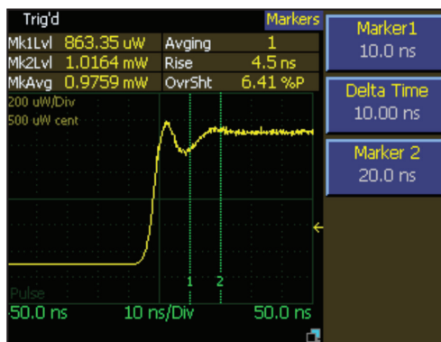
Figure 6.2.2. Power vs. Time trace of the rising edge of a Peak Power Envelope
