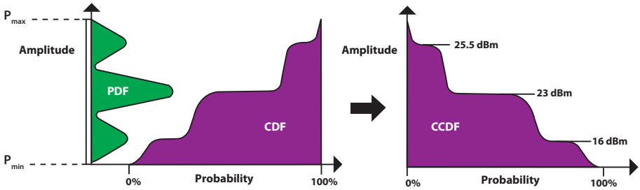
Figure 6.3.1. Common statistical diagrams including a PDF, CDF and CCDF
