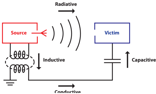
Figure 7.3.1. Electromagnetic Coupling paths
