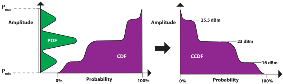
Figure 7.2.3. PDF, CDF, and CCDF diagram
