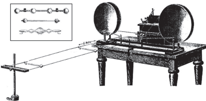
Ernst Lecher's apparatus for measuring RF amplitude
