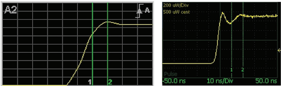
Figure 6.2.5. Screen shot of under-sampled rising edge on left and well-defined, over-sampled edge on right
