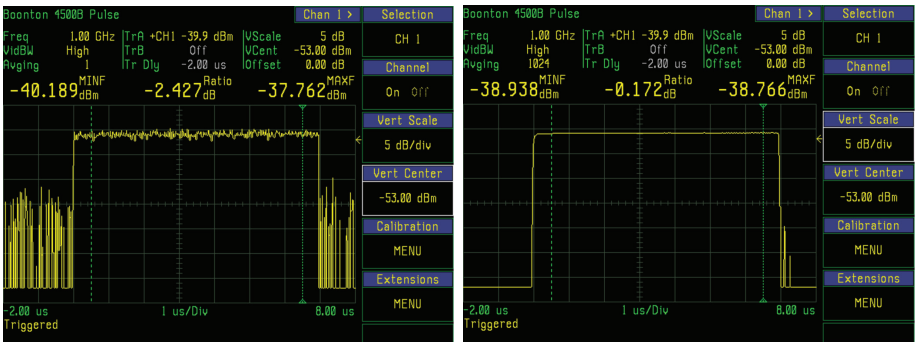
8.1.2 Effect of trace averaging for reducing noise on periodic pulse waveform. These screen shots both show one low-level (-39dBm) pulse of a periodic waveform. The left trace has no averaging, and its min-to-max ratio is about 2.4 dB, representing the effective peak-to-peak measurement noise. Increasing averaging to 1024 in the right trace reduces peak-to-peak noise during the pulse to less than 0.2dB, as well as bringing the noise floor down from about -53dBm to below -70dBm.
