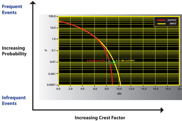
Figure 7.2.6. Dual CCDF “input/output” display shows the output has a reduced crest factor, indicating signal compression
